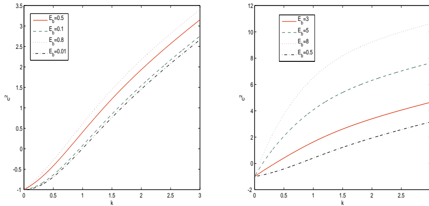
Fig. 2. Linear dispersion relation (26) as the electric field strength parameter E_b varies from small values (left panel) to moderate values (right panel). Other parameters are B = 1 , \epsilon_{s,f} = 0.5 , \epsilon_{f,g} = 3 . The band of instability decreases as E_b increases.
