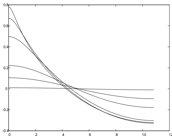
Fig. 4. Wave profiles for E_b = 8 , \epsilon_{s,f} = 0.5 , \epsilon_{f,g} = 3 , \lambda = 21.7 and various values of h .
